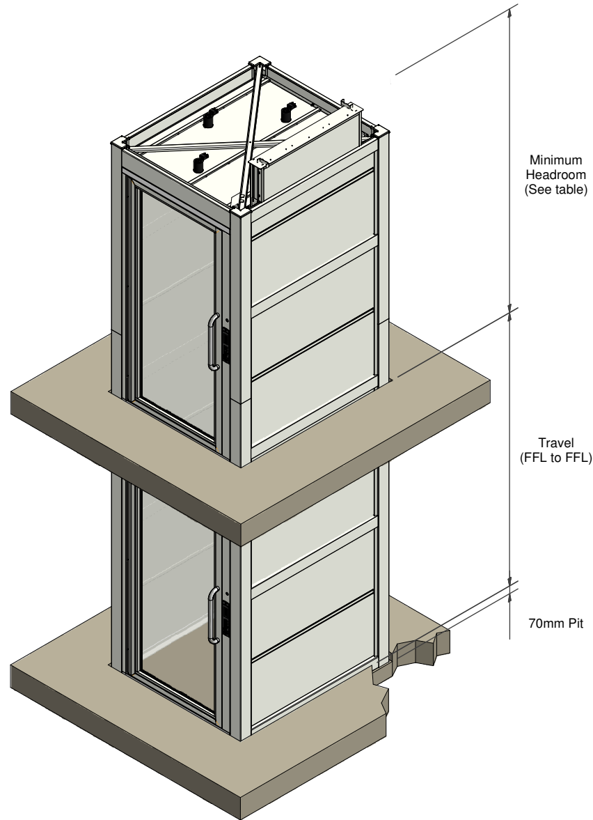
Door at Upper Level (travel 300 to 7000mm)
